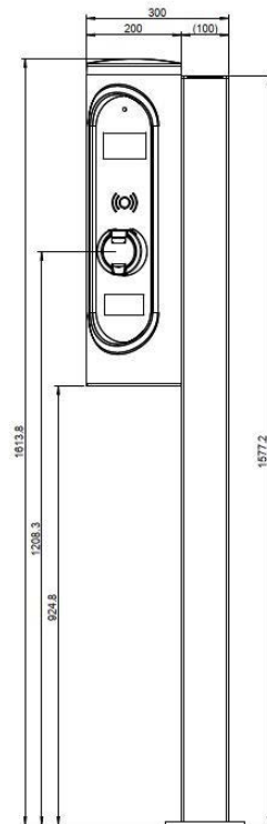
Dimension sketch
